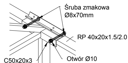
Detail F
