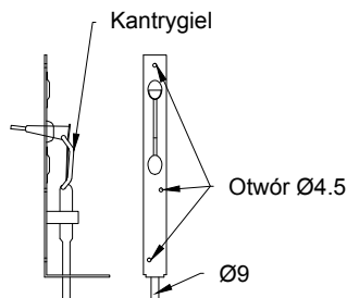
Detail H
